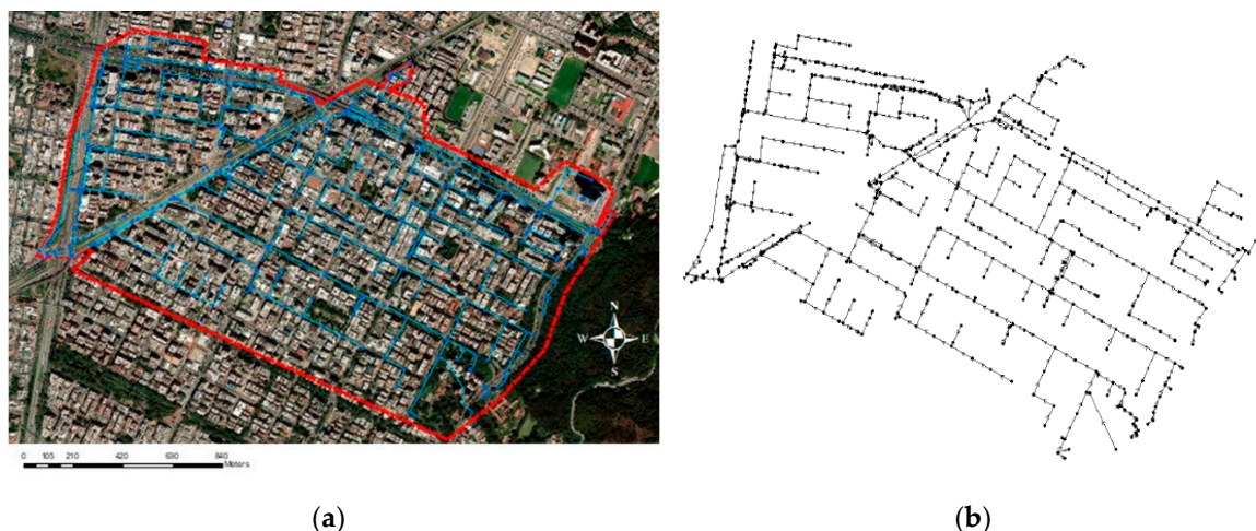
Figure 5. (a) Location of Southern Chicó Network. (b) Storm Water Management Model (SWMM) for Southern Chicó Network.
